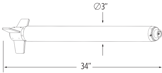
Explorator Tow Fish 8.5 lbs in air, 2.6 lbs in water
