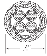
Up to 150m Tow Cable 0.082 lb/1000 ft in air 0.023 lb/1000 ft in water
